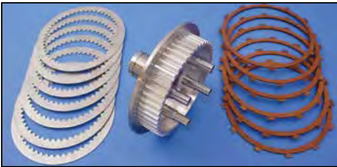
1984-89 Big Twin Clutch Hub Kit includes updated reinforced steel center clutch hub, steel drive plate set and friction plate set. VT No. 18-0541
